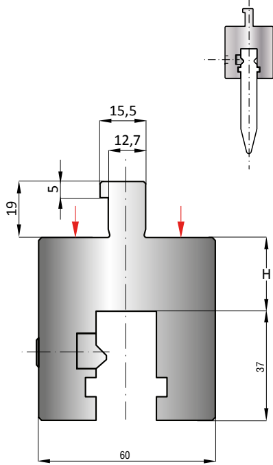
ADATTATORE- ADAPTER - ADAPTADORE ADAPTADORE - ADAPTATEUR - ADAPTER USA - EU / WILA ADAPTER
