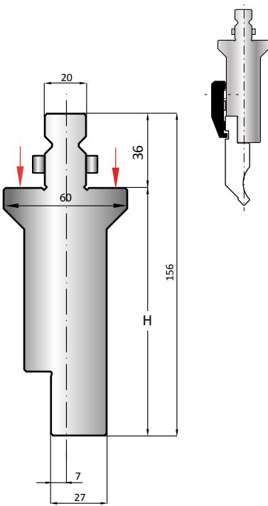
ADATTATORE- ADAPTER - ADAPTADORE ADAPTADORE - ADAPTATEUR - ADAPTER WILA - TRUMPF/ AMADA
