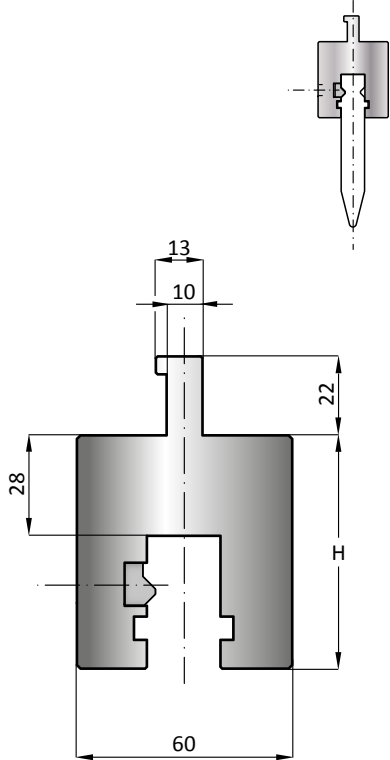
ADATTATORE- ADAPTER - ADAPTADORE ADAPTADORE - ADAPTATEUR - ADAPTER LVD / WILA - TRUMPF
