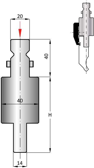
ADATTATORE- ADAPTER - ADAPTADORE ADAPTADORE - ADAPTATEUR - ADAPTER WILA - TRUMPF / AMADA
