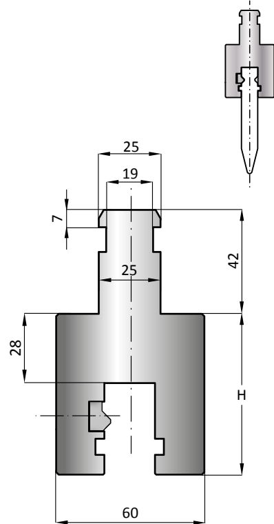
ADATTATORE- ADAPTER - ADAPTADORE ADAPTADORE - ADAPTATEUR - ADAPTER WEINBRENNER / WILA - TRUMPF
